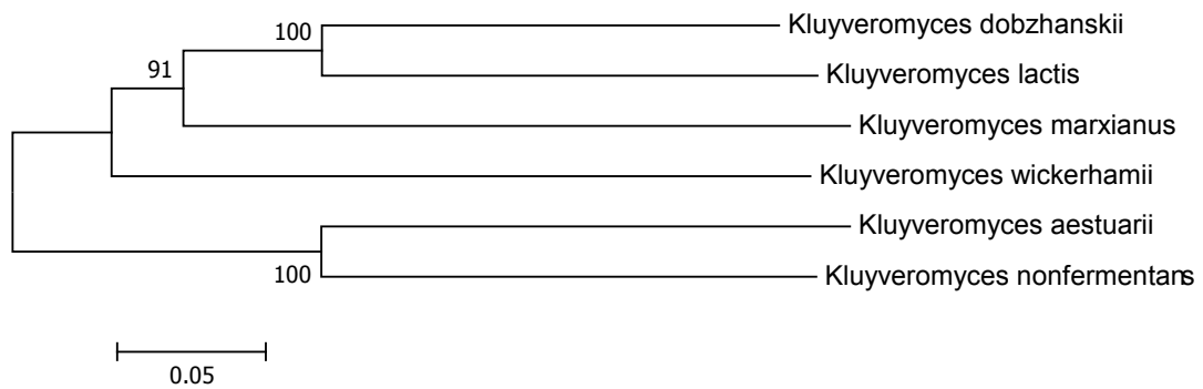
Kluyveromyces telomerase RNA
